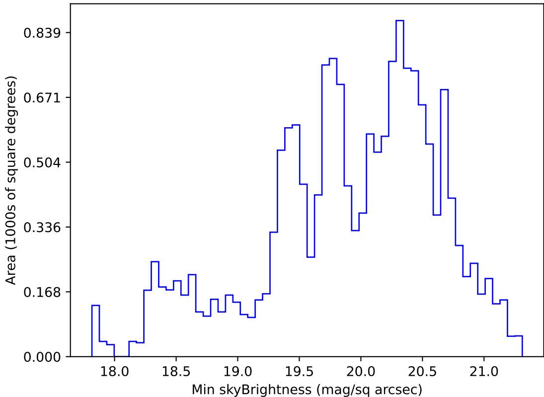
ddf_acor_sf10_lsf40_lsr20_v3.4_10yrs WFD g band: Min skyBrightness
