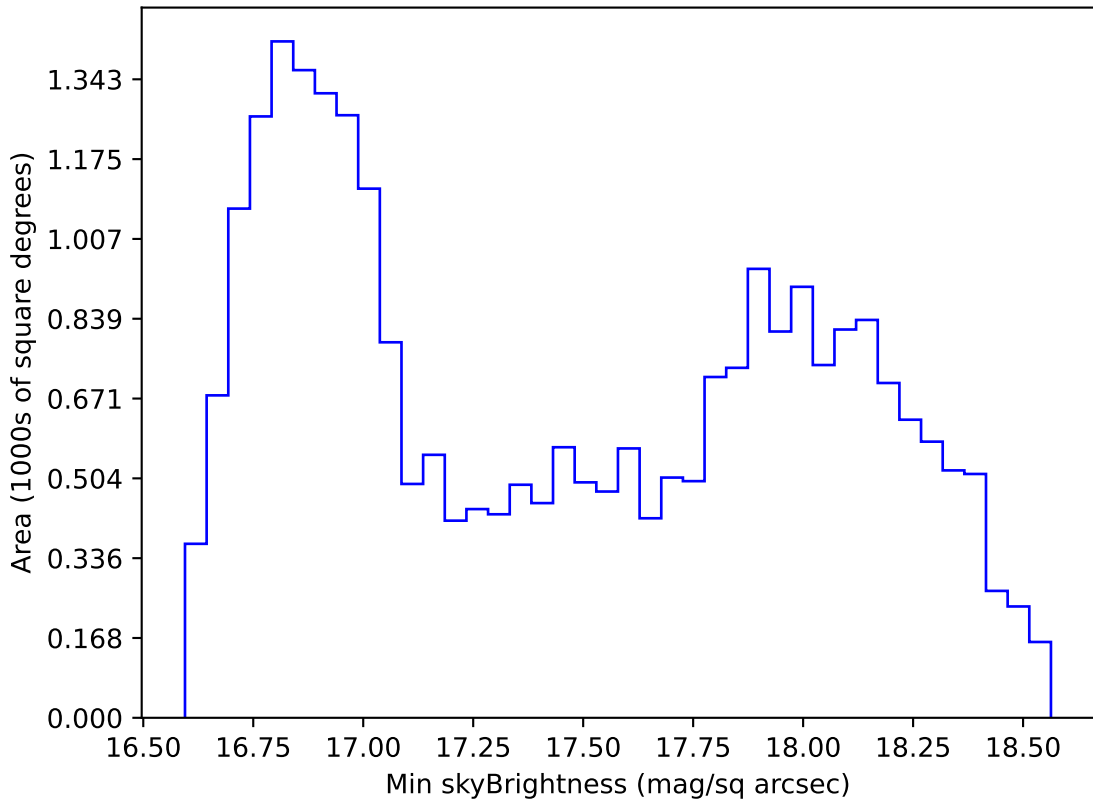
ddf_acor_sf10_lsf40_lsr20_v3.4_10yrs All sky z band: Min skyBrightness
