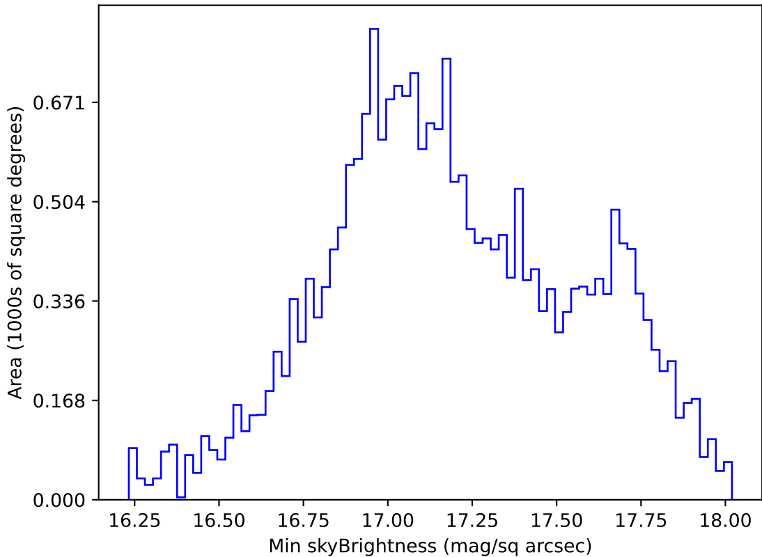
ddf_acor_sf10_lsf40_lsr20_v3.4_10yrs All sky y band: Min skyBrightness
