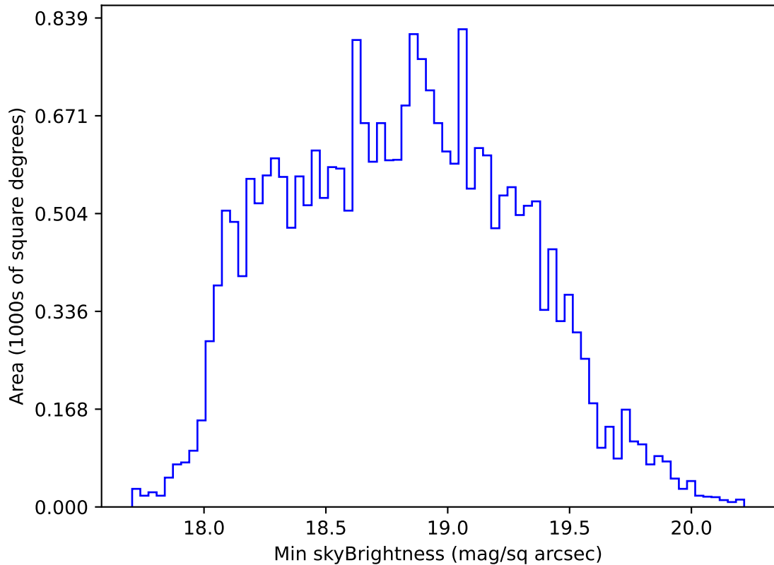
ddf_acor_sf10_lsf40_lsr20_v3.4_10yrs All sky r band: Min skyBrightness
