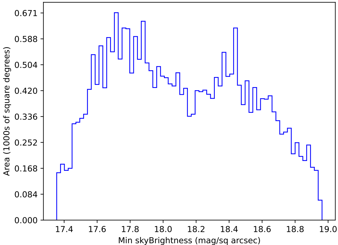
ddf_acor_sf10_lsf40_lsr20_v3.4_10yrs All sky i band: Min skyBrightness
