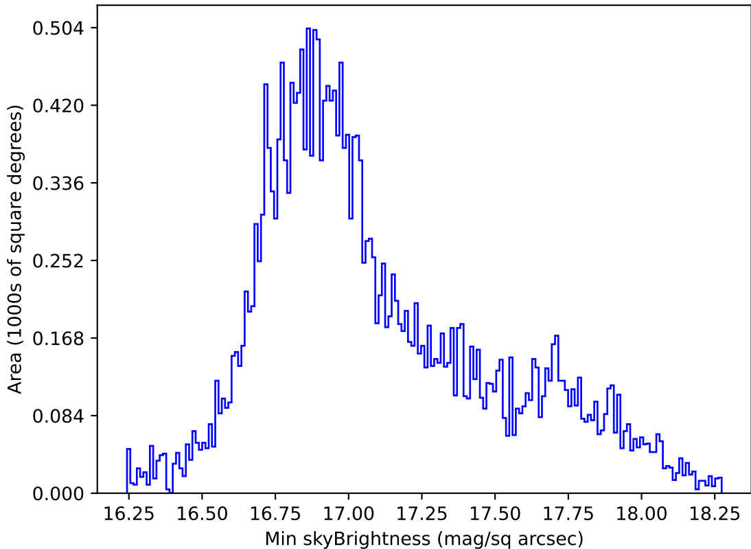
ddf_acor_sf10_lsf40_lsr20_v3.4_10yrs All sky all bands: Min skyBrightness
