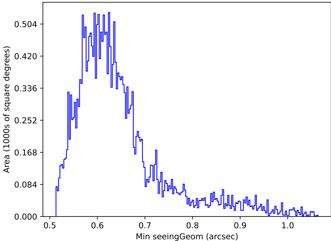
ddf_acor_sf10_ls40_lsr20_v3.4_10yrs Yr 1 z band: Min seeingGeom
