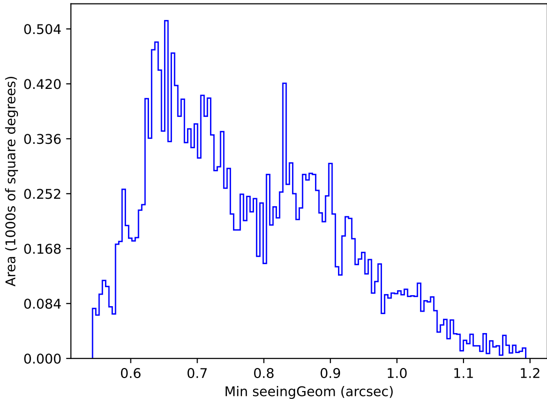
ddf_acor_sf10_ls40_lsr20_v3.4_10yrs Yr 1 u band: Min seeingGeom
