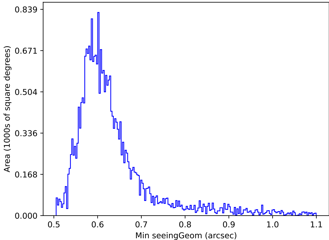
ddf_acor_sf10_lsf40_lsr20_v3.4_10yrs Yr 1 i band: Min seeingGeom
