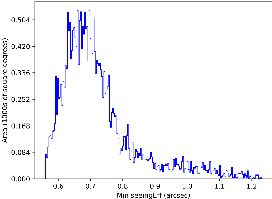
ddf_acor_sf10_lsf40_lsr20_v3.4_10yrs Yr 1 z band: Min seeingEff
