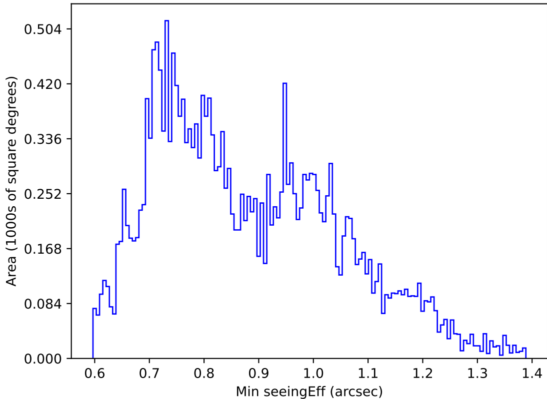
ddf_acor_sf10_lsf40_lsr20_v3.4_10yrs Yr 1 u band: Min seeingEff
