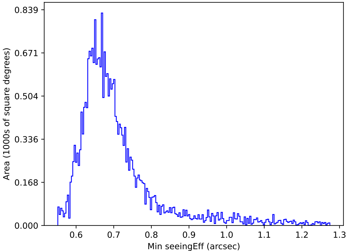
ddf_acor_sf10_lsf40_lsr20_v3.4_10yrs Yr 1 i band: Min seeingEff
