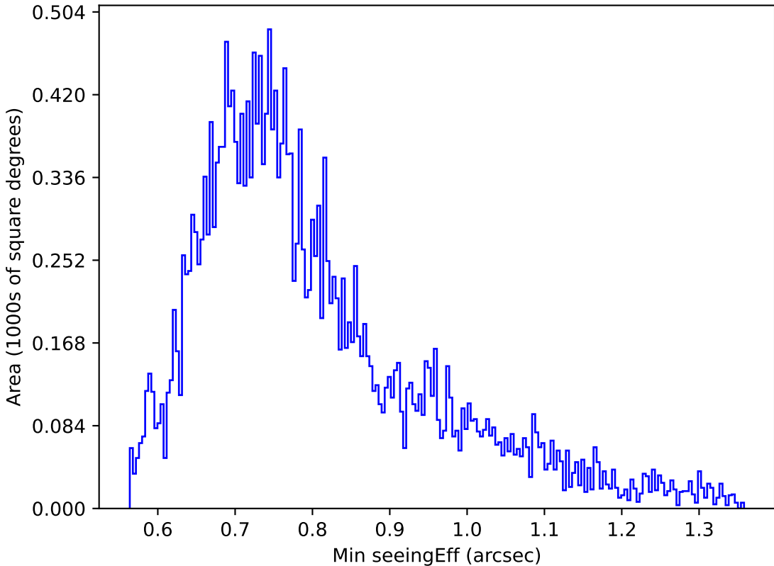
ddf_acor_sf10_lsf40_lsr20_v3.4_10yrs Yr 1 g band: Min seeingEff
