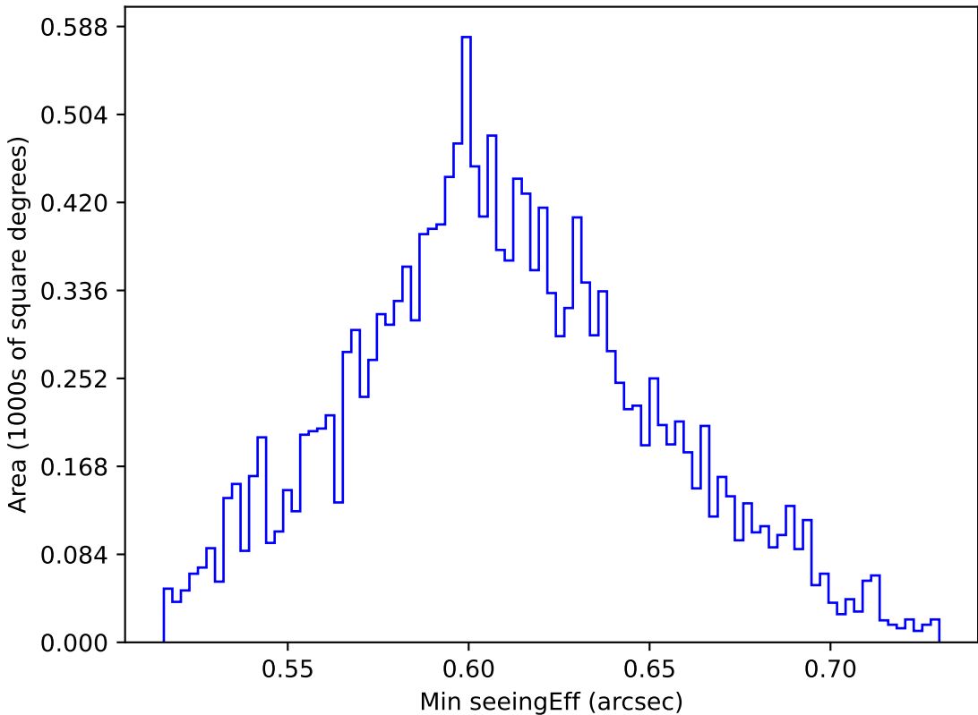
ddf_acor_sf10_lsf40_lsr20_v3.4_10yrs WFD z band: Min seeingEff
