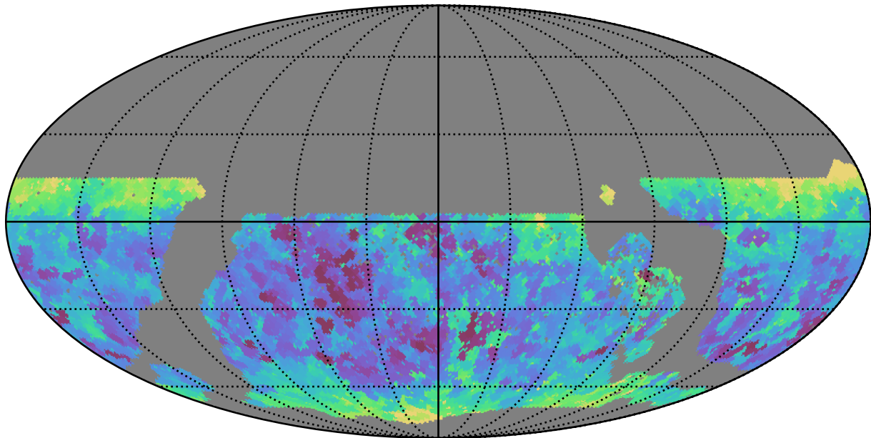
ddf_acor_sf10_lsf40_lsr20_v3.4_10yrs WFD y band: Min seeingEff
