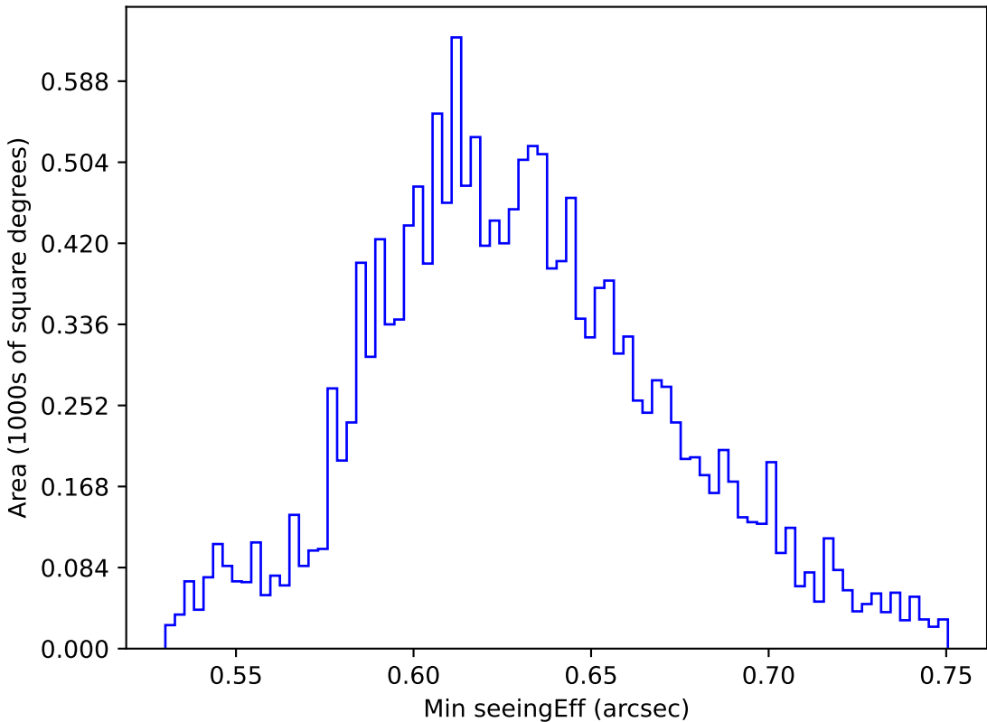
ddf_acor_sf10_lsf40_lsr20_v3.4_10yrs WFD y band: Min seeingEff
