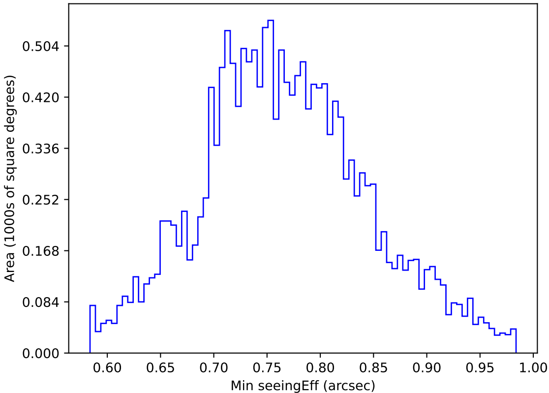
ddf_acor_sf10_lsf40_lsr20_v3.4_10yrs WFD u band: Min seeingEff
