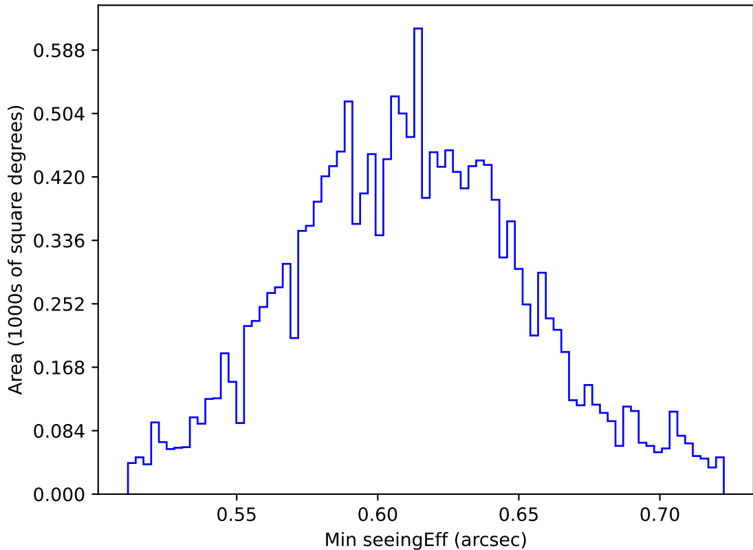
ddf_acor_sf10_lsf40_lsr20_v3.4_10yrs WFD r band: Min seeingEff
