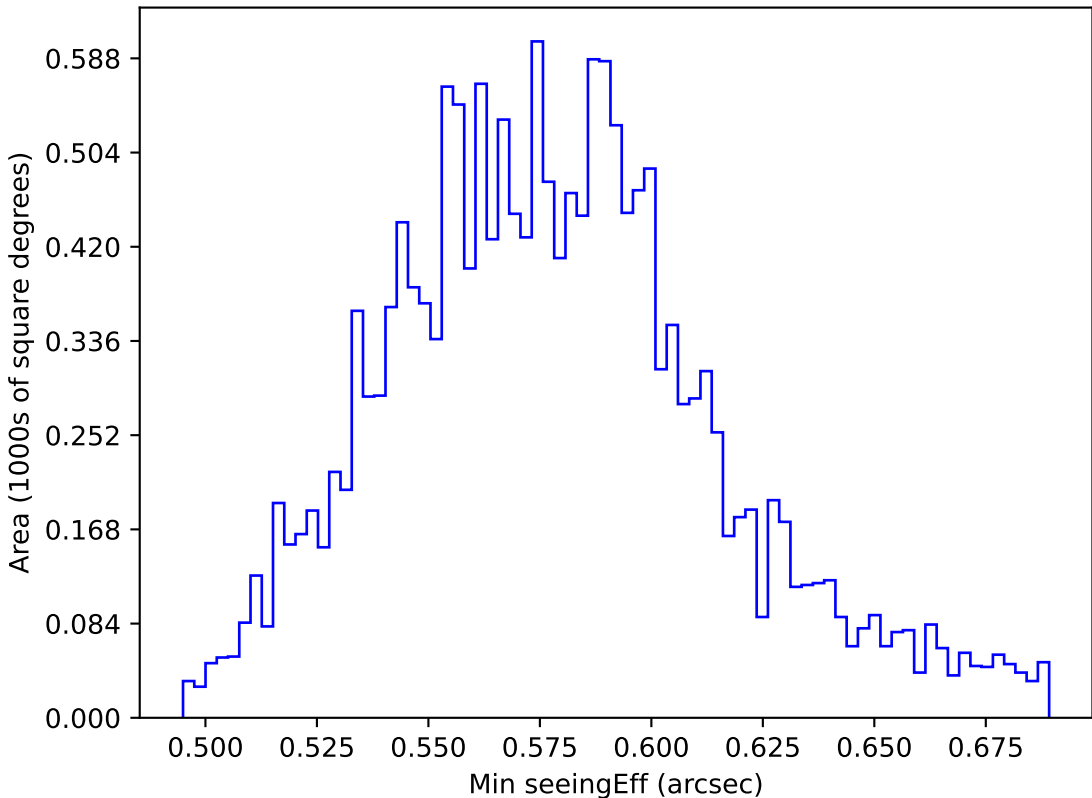
ddf_acor_sf10_ls40_lsr20_v3.4_10yrs WFD all bands: Min seeingEff
