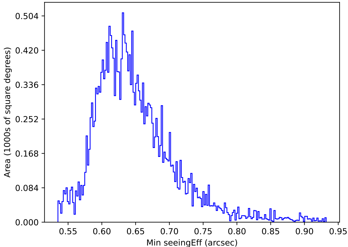
ddf_acor_sf10_lsf40_lsr20_v3.4_10yrs All sky y band: Min seeingEff
