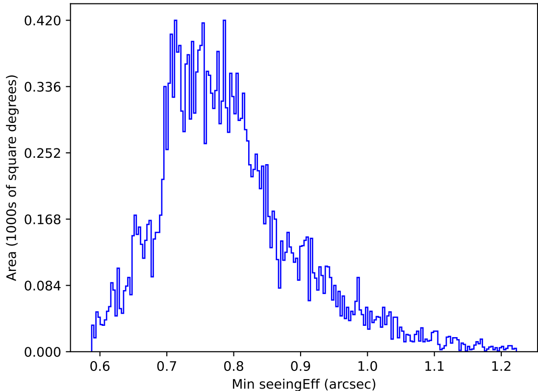
ddf_acor_sf10_lsf40_lsr20_v3.4_10yrs All sky u band: Min seeingEff
