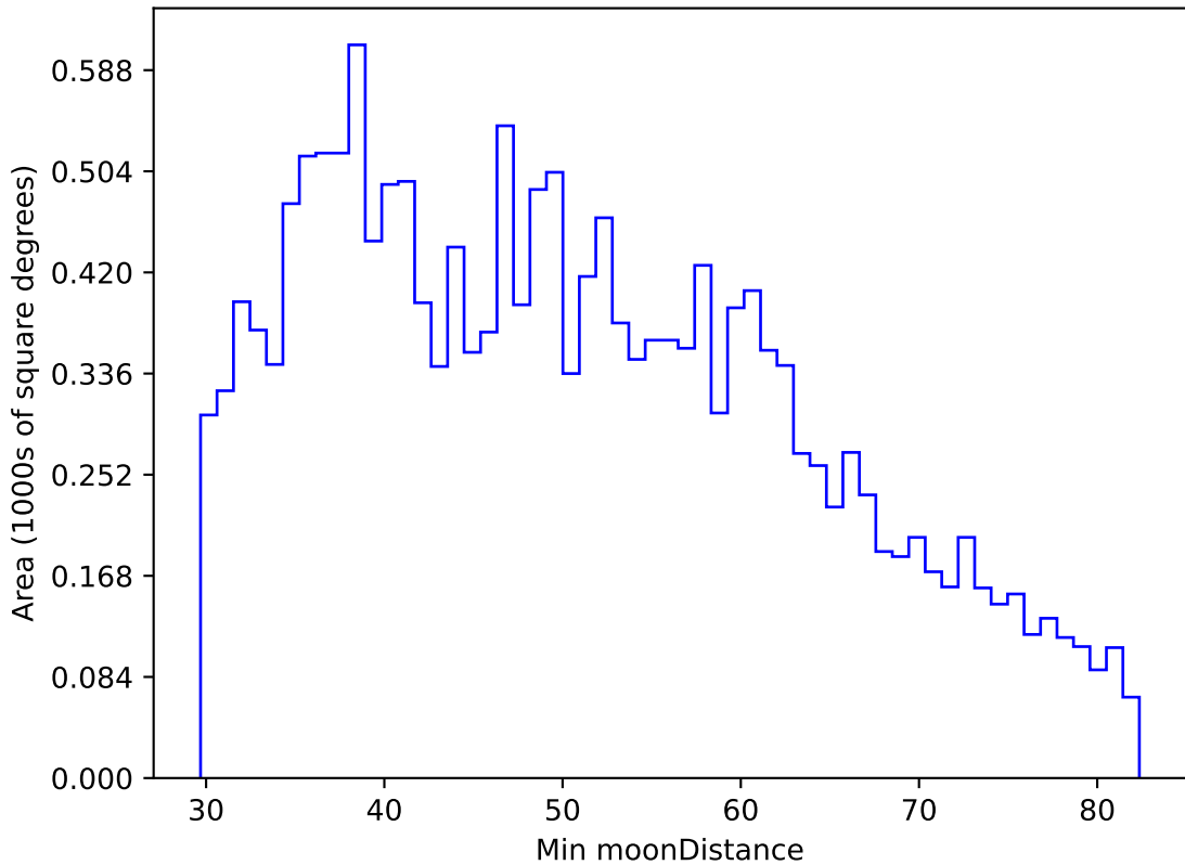
ddf_acor_sf10_lsf40_lsr20_v3.4_10yrs WFD u band: Min moonDistance
