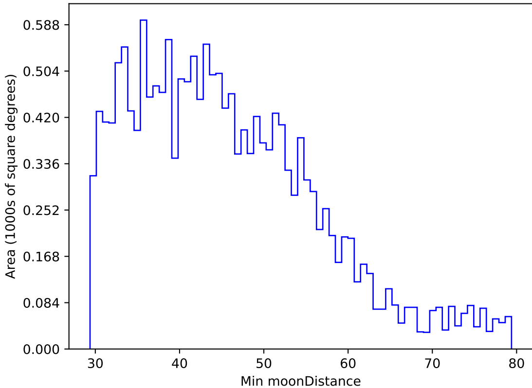
ddf_acor_sf10_lsf40_lsr20_v3.4_10yrs WFD g band: Min moonDistance
