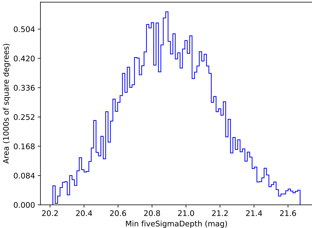
ddf_acor_sf10_lsf40_lsr20_v3.4_10yrs All sky y band: Min fiveSigmaDepth
