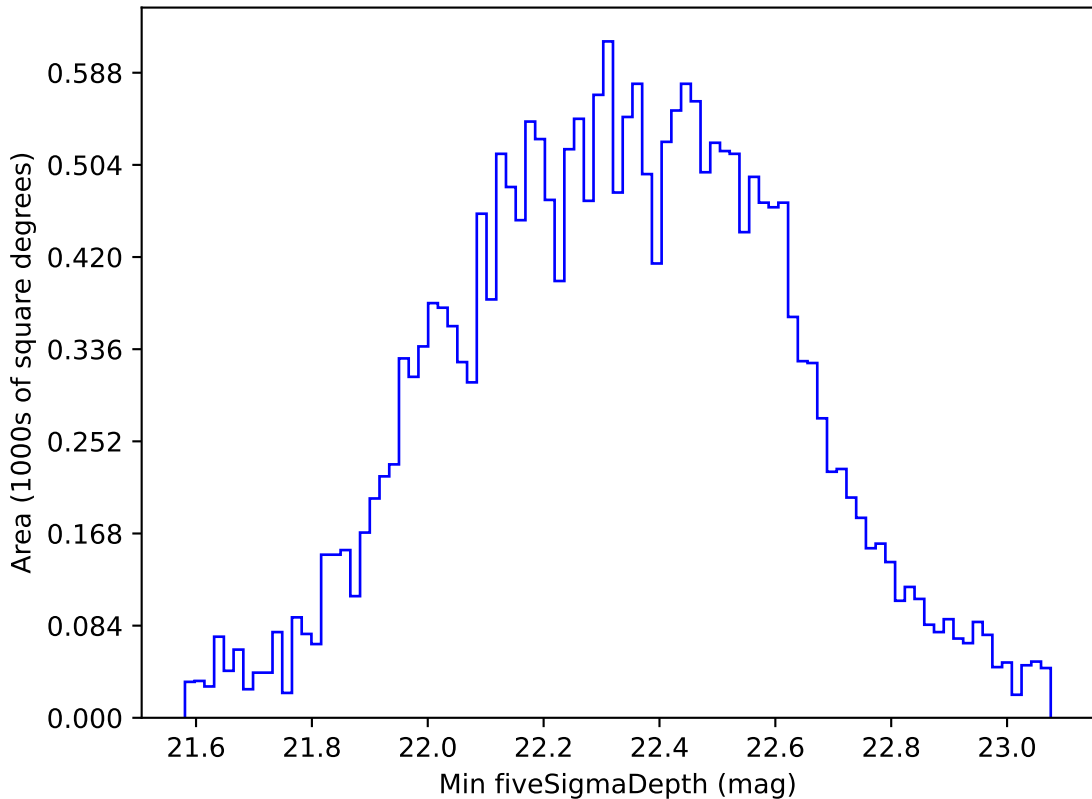
ddf_acor_sf10_lsf40_lsr20_v3.4_10yrs All sky u band: Min fiveSigmaDepth
