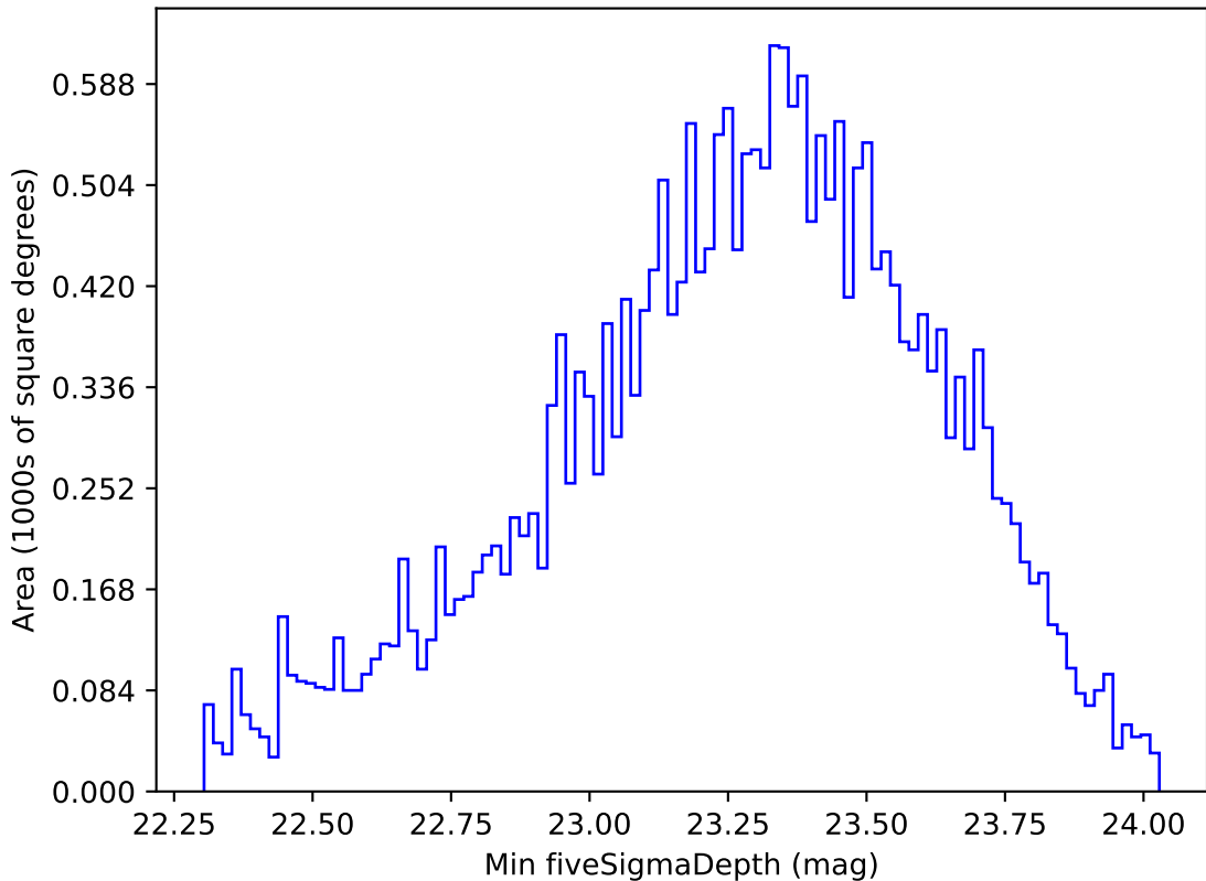
ddf_acor_sf10_lsf40_lsr20_v3.4_10yrs All sky g band: Min fiveSigmaDepth
