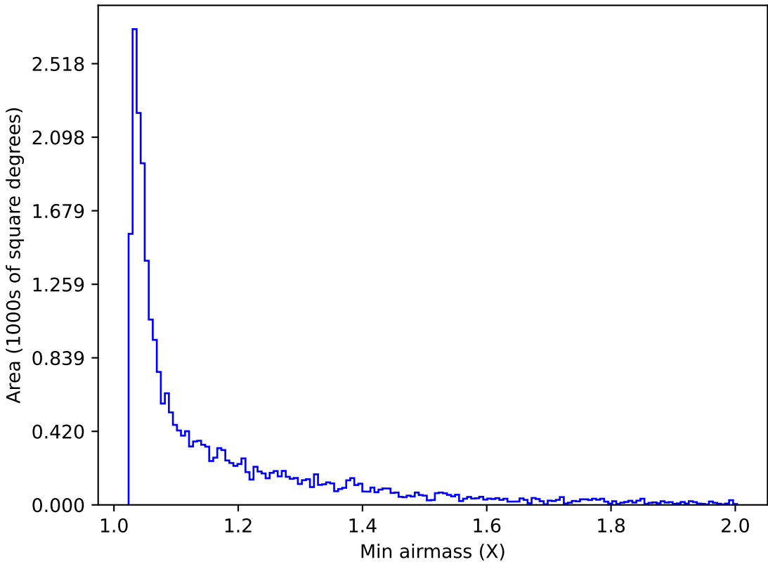
ddf_acor_sf10_lsf40_lsr20_v3.4_10yrs Yr 1 z band: Min airmass
