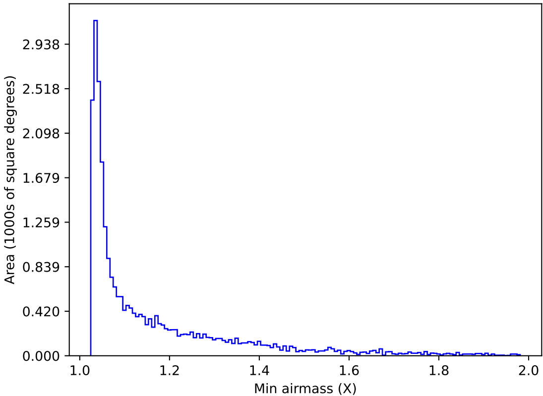
ddf_acor_sf10_lsf40_lsr20_v3.4_10yrs Yr 1 i band: Min airmass
