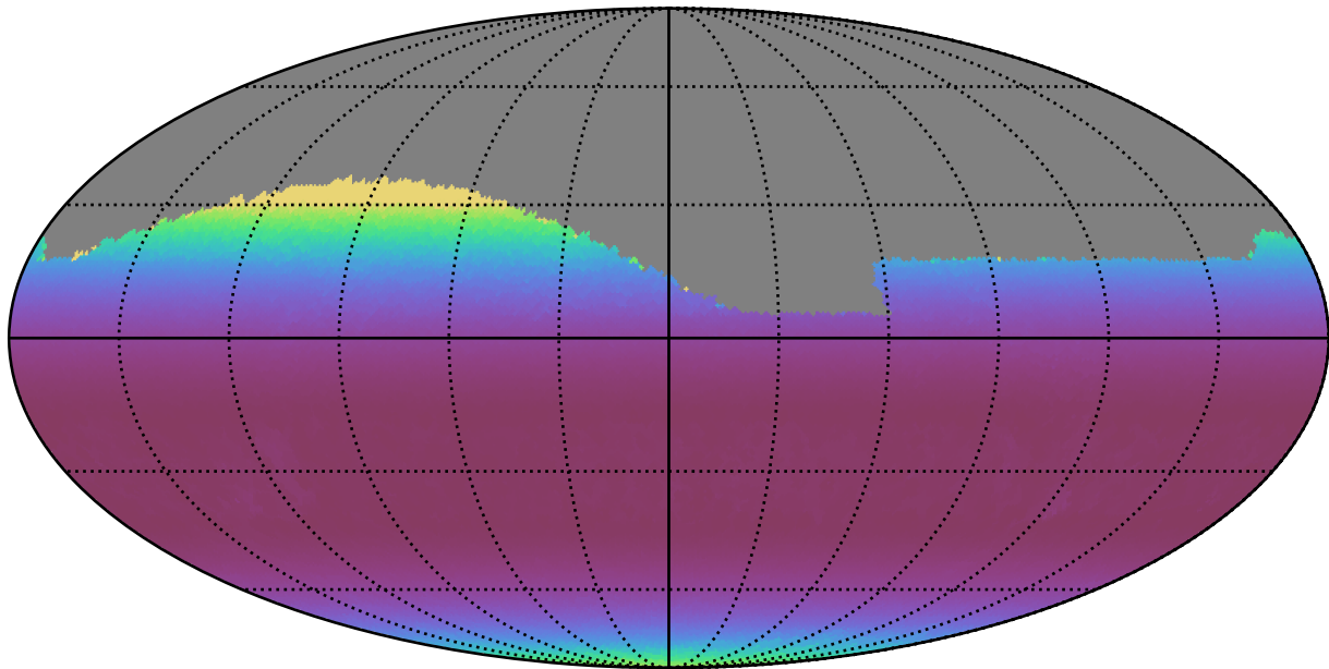
ddf_acor_sf10_lsf40_lsr20_v3.4_10yrs Yr 1 all bands: Min airmass
