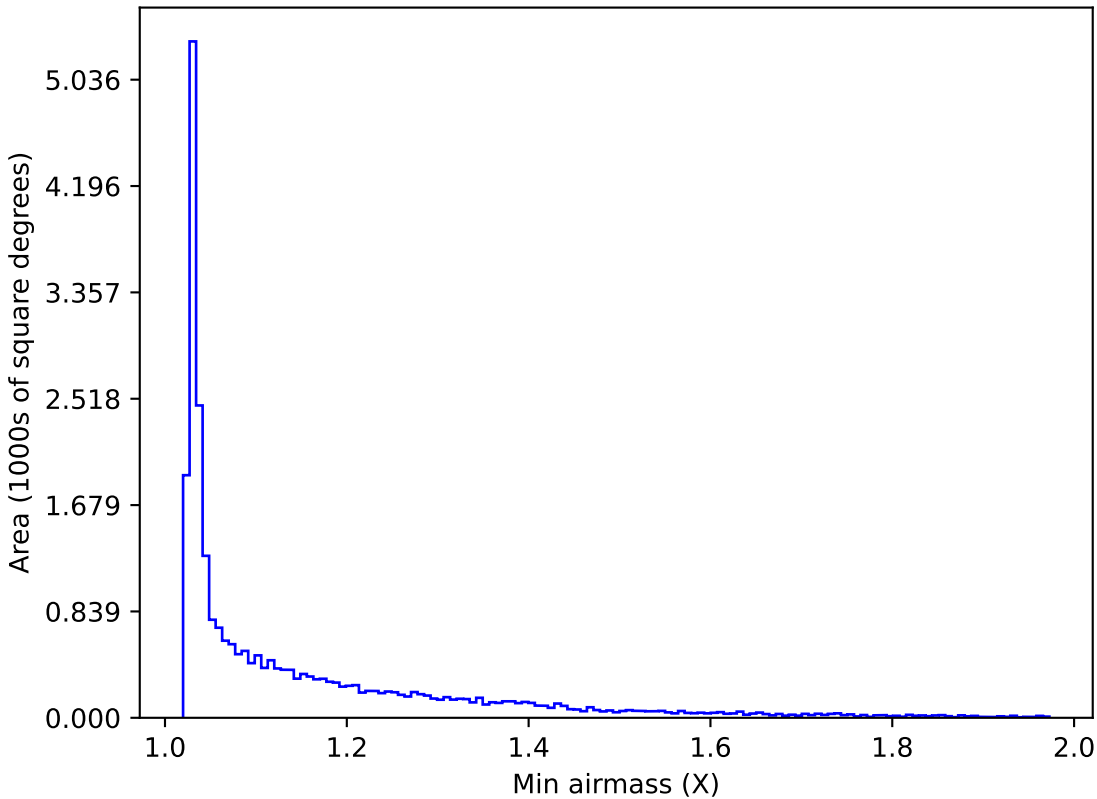
ddf_acor_sf10_lsf40_lsr20_v3.4_10yrs Yr 1 all bands: Min airmass
