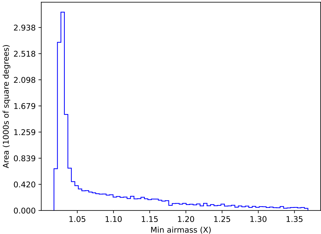
ddf_acor_sf10_lsf40_lsr20_v3.4_10yrs WFD z band: Min airmass
