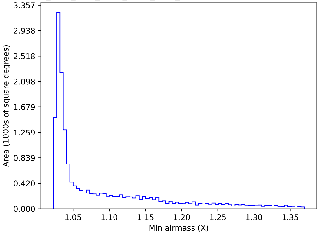
ddf_acor_sf10_lsf40_lsr20_v3.4_10yrs WFD y band: Min airmass
