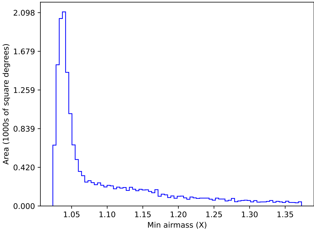
ddf_acor_sf10_lsf40_lsr20_v3.4_10yrs WFD u band: Min airmass
