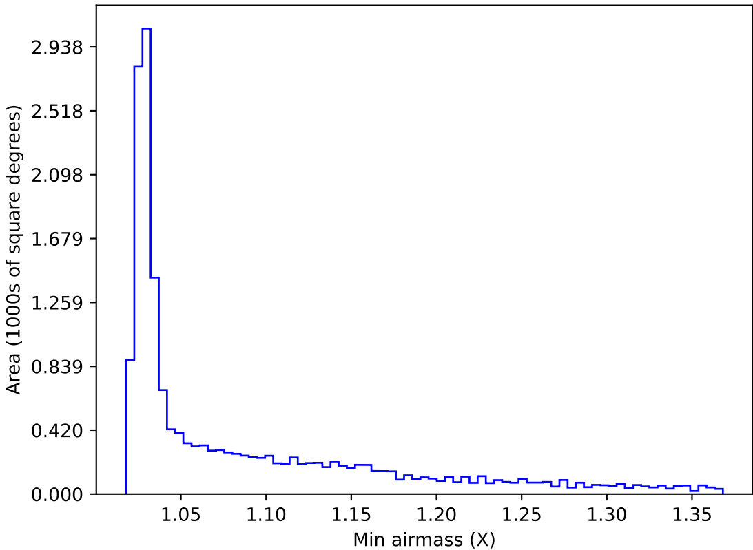
ddf_acor_sf10_lsf40_lsr20_v3.4_10yrs WFD i band: Min airmass
