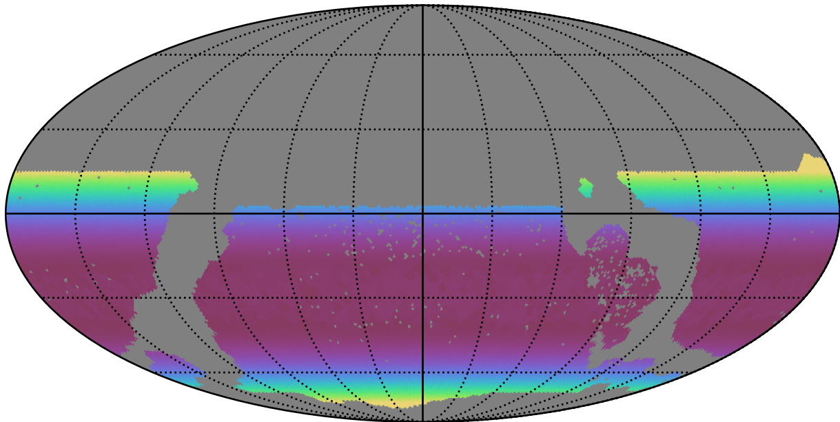
ddf_acor_sf10_lsf40_lsr20_v3.4_10yrs WFD all bands: Min airmass
