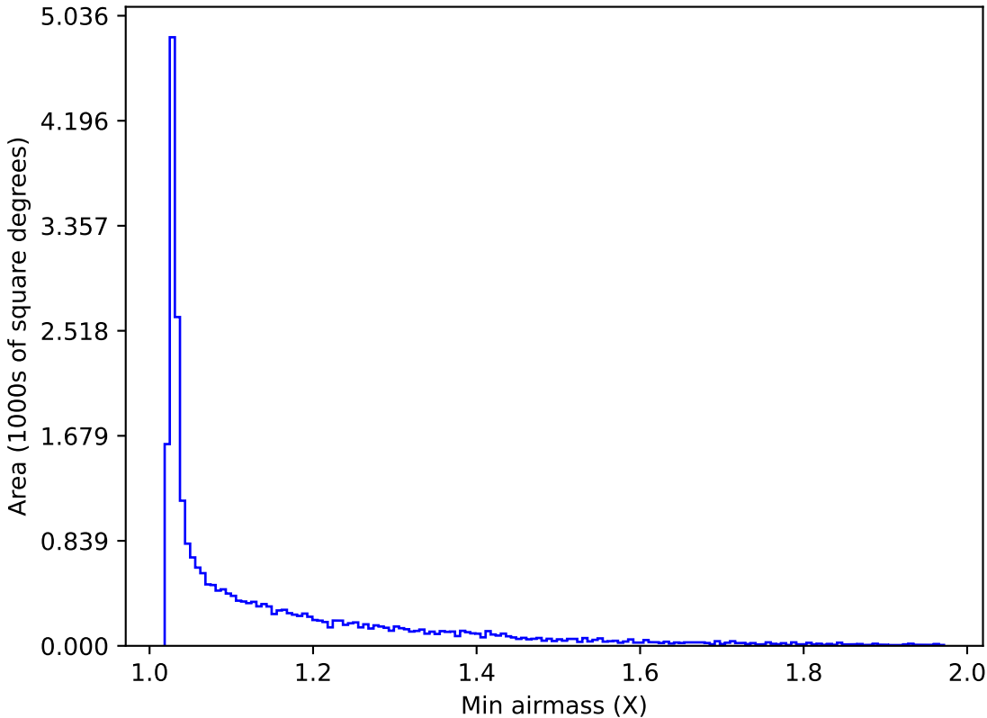
ddf_acor_sf10_lsf40_lsr20_v3.4_10yrs All sky z band: Min airmass
