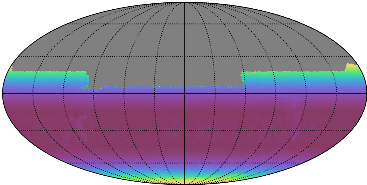
ddf_acor_sf10_lsf40_lsr20_v3.4_10yrs All sky y band: Min airmass
