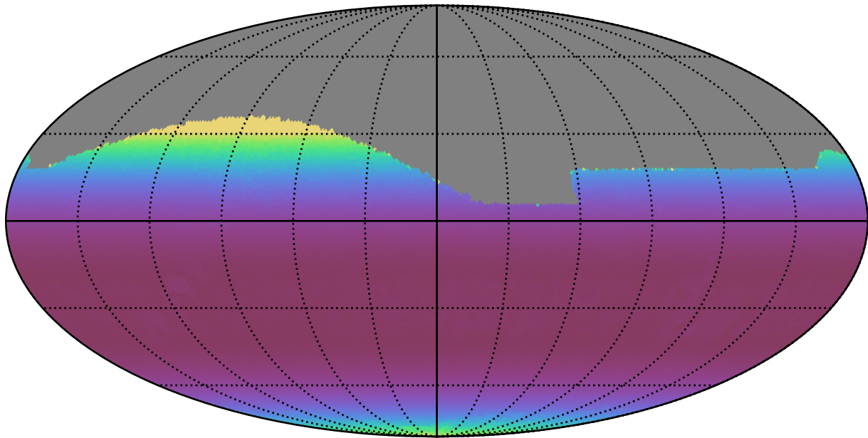
ddf_acor_sf10_lsf40_lsr20_v3.4_10yrs All sky r band: Min airmass
