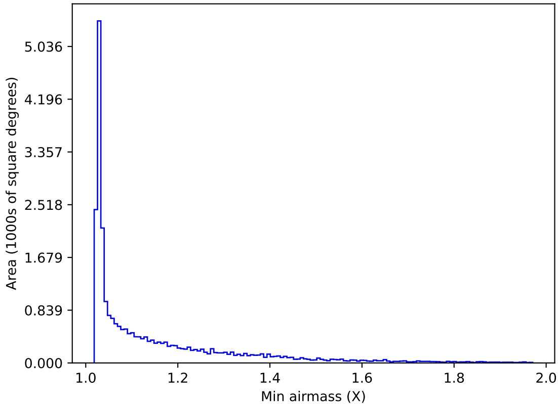
ddf_acor_sf10_lsf40_lsr20_v3.4_10yrs All sky i band: Min airmass
