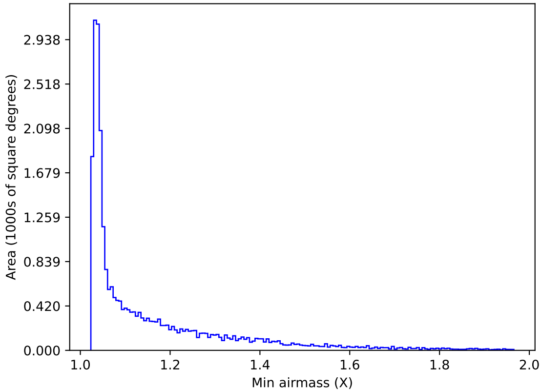
ddf_acor_sf10_lsf40_lsr20_v3.4_10yrs All sky g band: Min airmass
