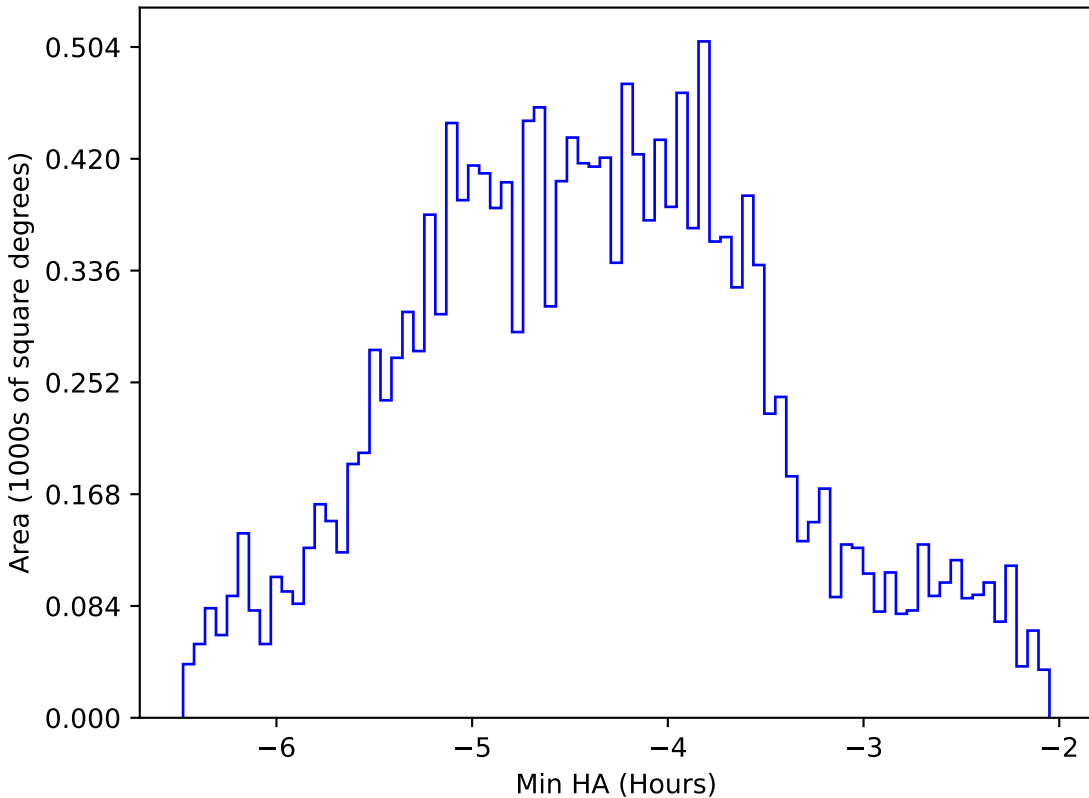
ddf_acor_sf10_lsf40_lsr20_v3.4_10yrs WFD z band: Min HA
