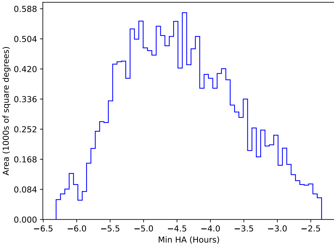
ddf_acor_sf10_lsf40_lsr20_v3.4_10yrs WFD r band: Min HA
