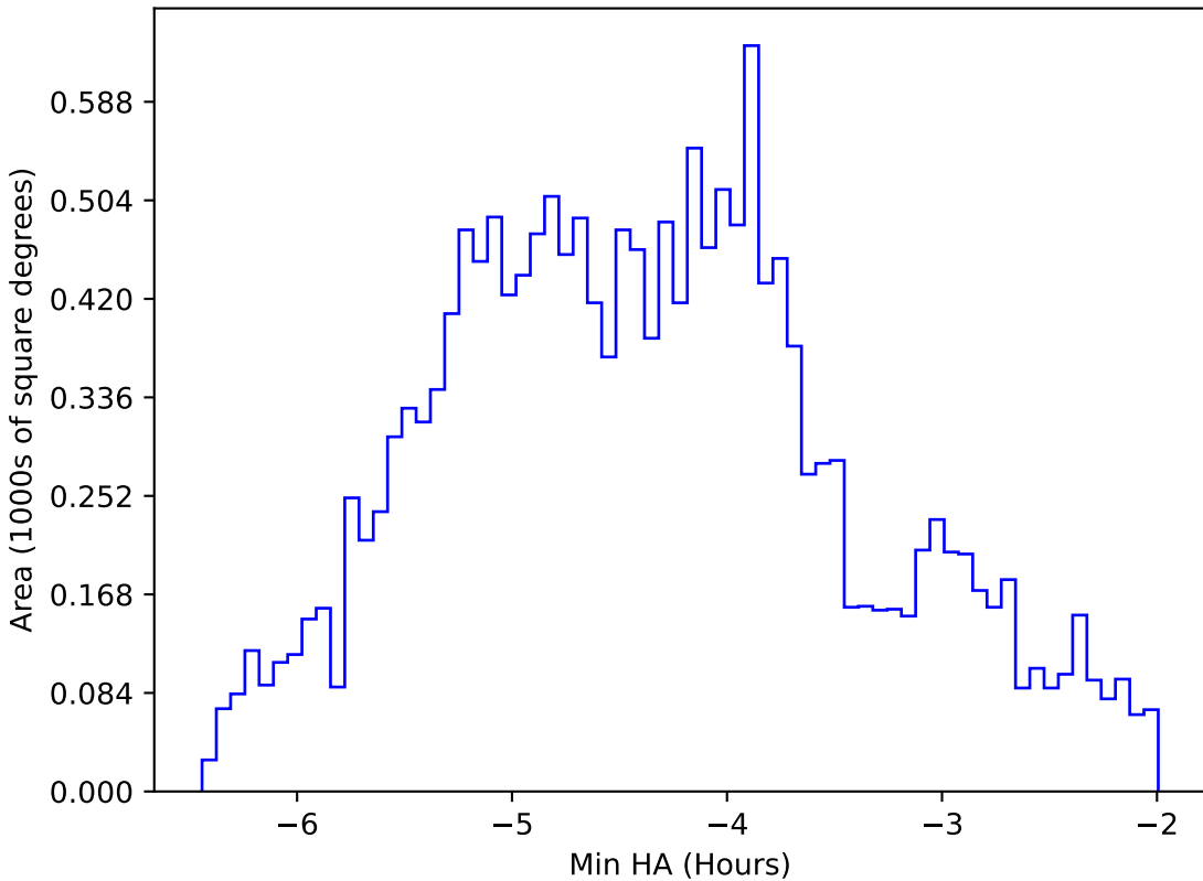
ddf_acor_sf10_lsf40_lsr20_v3.4_10yrs WFD i band: Min HA
