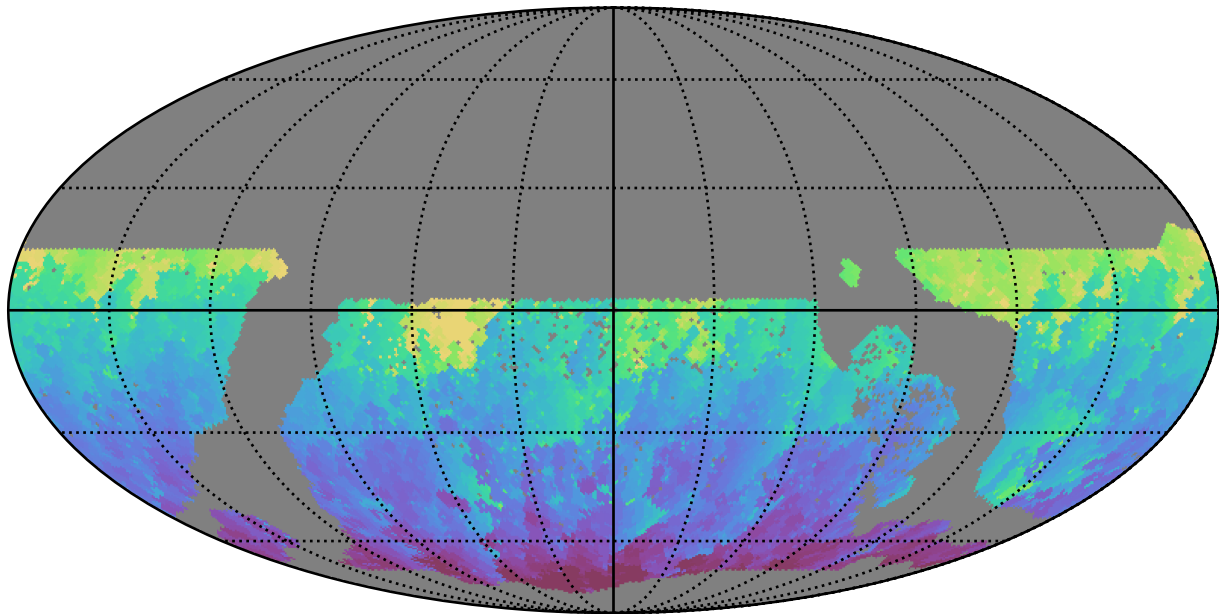
ddf_acor_sf10_lsf40_lsr20_v3.4_10yrs WFD g band: Min HA
