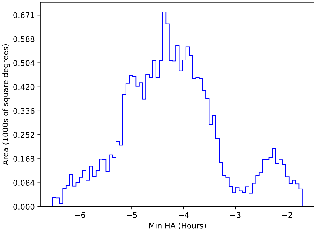
ddf_acor_sf10_lsf40_lsr20_v3.4_10yrs WFD g band: Min HA
