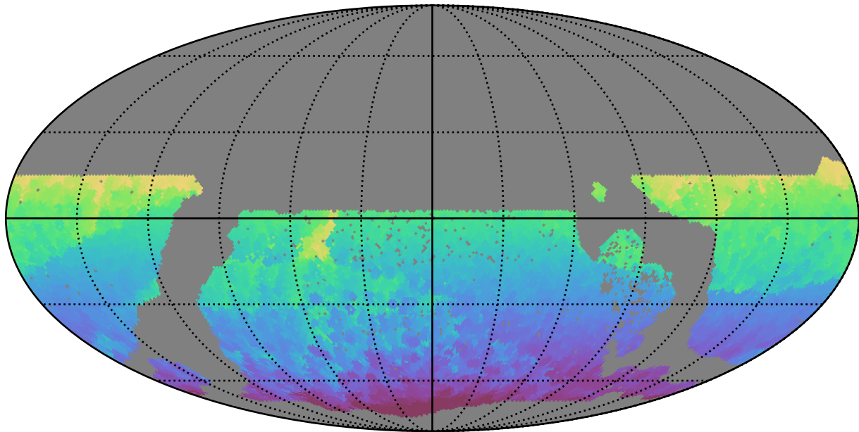
ddf_acor_sf10_lsf40_lsr20_v3.4_10yrs WFD all bands: Min HA
