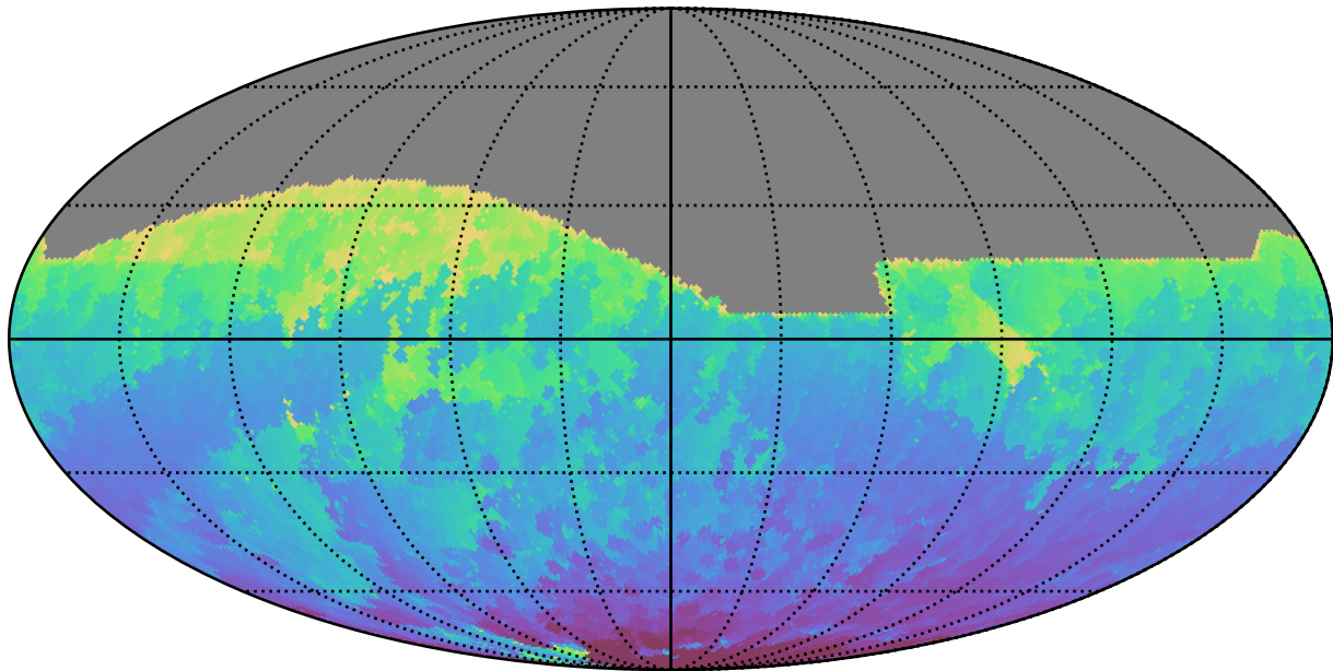
ddf_acor_sf10_lsf40_lsr20_v3.4_10yrs All sky z band: Min HA
