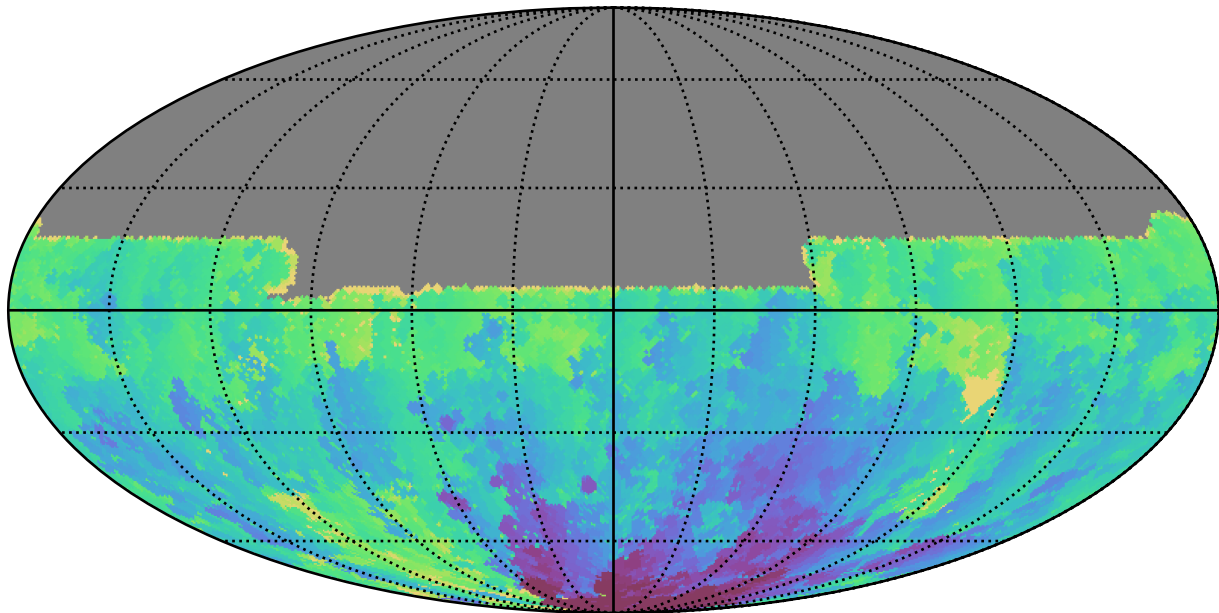
ddf_acor_sf10_lsf40_lsr20_v3.4_10yrs All sky u band: Min HA
