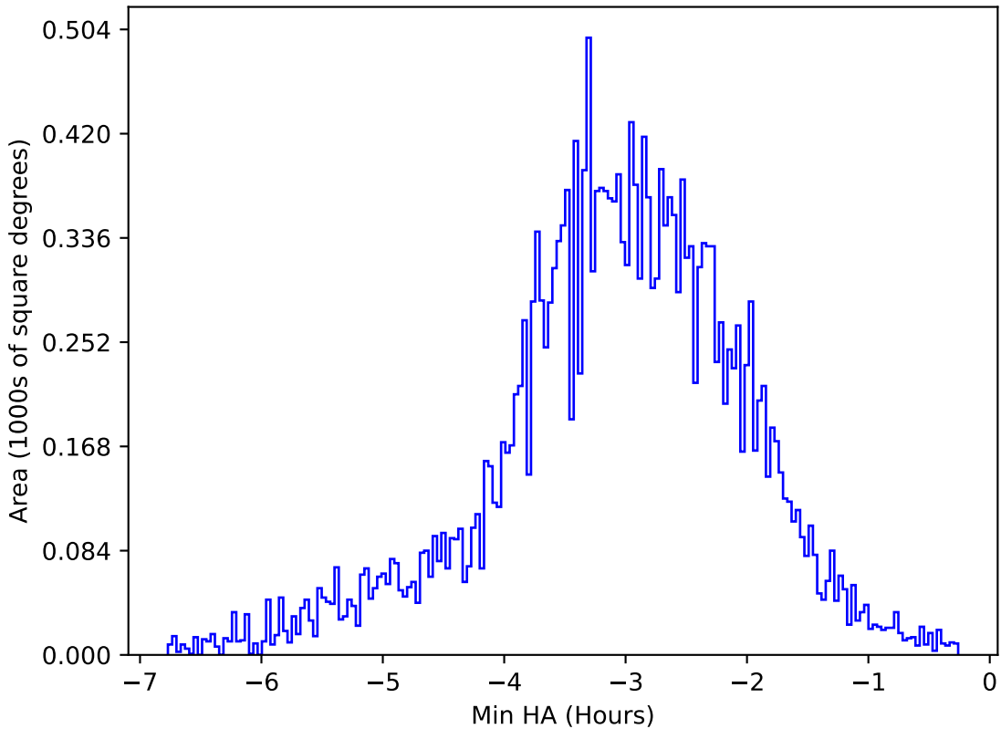
ddf_acor_sf10_lsf40_lsr20_v3.4_10yrs All sky u band: Min HA
