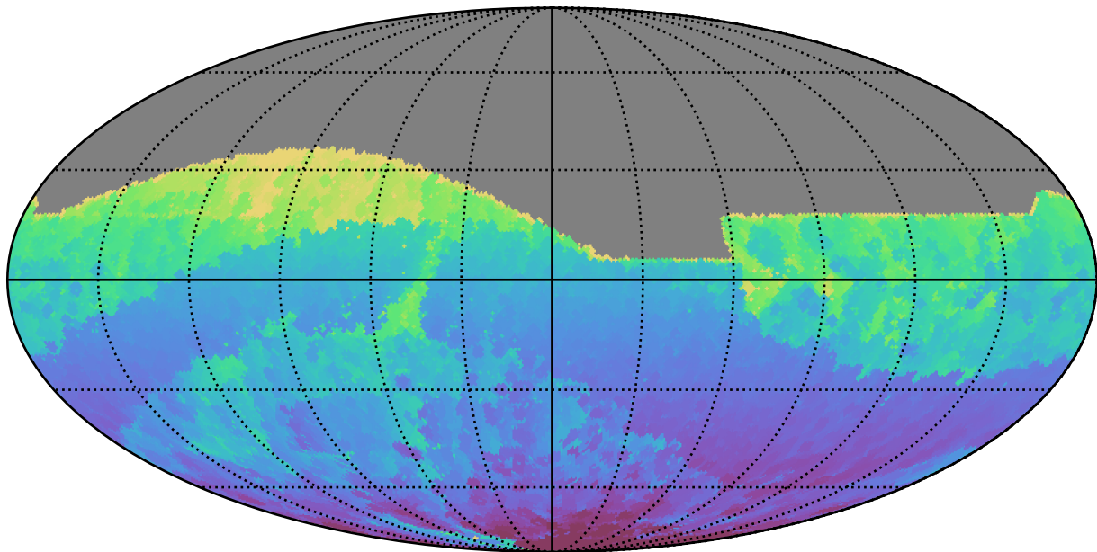
ddf_acor_sf10_lsf40_lsr20_v3.4_10yrs All sky r band: Min HA
